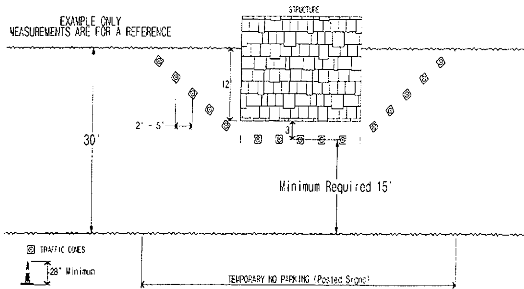
Temporary No Parking Diagram
