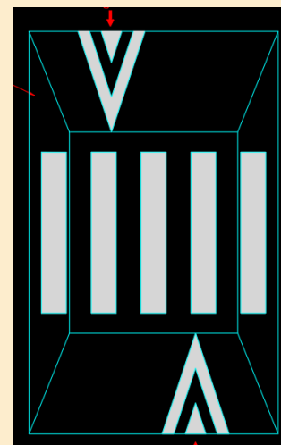
Raised Asphalt crosswalk diagram
